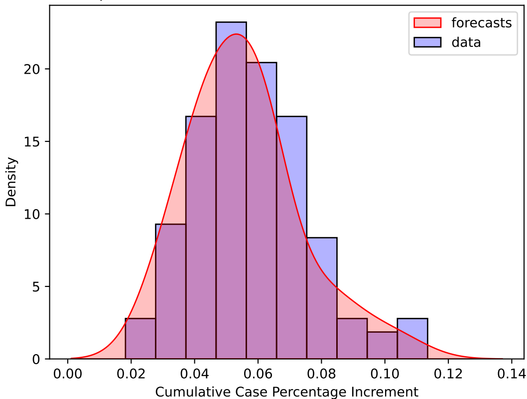
comparison between real data and forecasts at time 50
